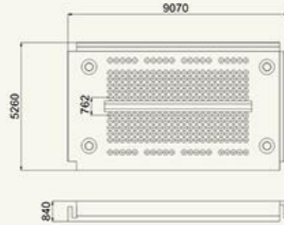
1 Terminal Strip, Tie-point 270 Board: 9*5.3*0.85(cm)
