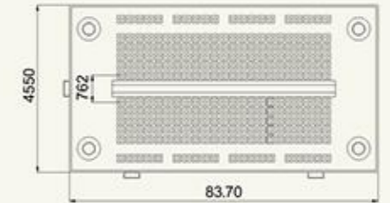
1 Terminal Strip,Tie-point270; Board:8.6*4.6*0.85(cm)
